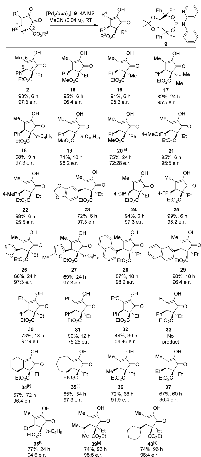
Scheme 2. Cyclization products with yields, completion times, and e.r. values. Unless otherwise noted, reaction conditions were as described in the Experimental Section. [a] Using ligand 5 , 82:18 e.r. (91%). With ligand 6 , 90:10 e.r. (77%). [b] [Pd 2 (dba) 3 ] (5 mol %) and 9 (15 mol %). [c] [Pd 2 (dba) 3 ] (15 mol %) and 9 (40 mol %). [d] [Pd 2 (dba) 3 ] (20 mol %) and 9 (50 mol %).
